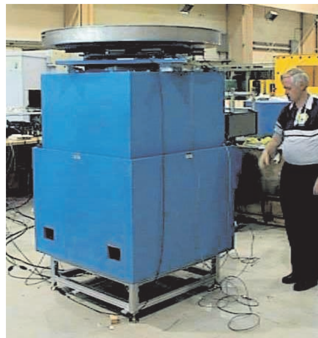
Fig. 5. Translator (prior to install)
