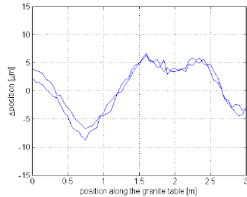
Figure 5: Effect of carriage pitch on probe z-position in 0.5 m height difference
